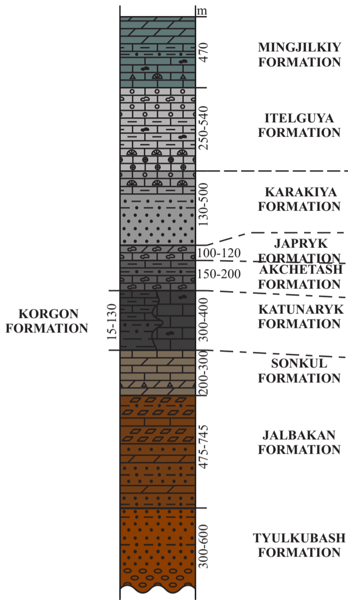
Generalized section after E. V. Khrstov (1970)
