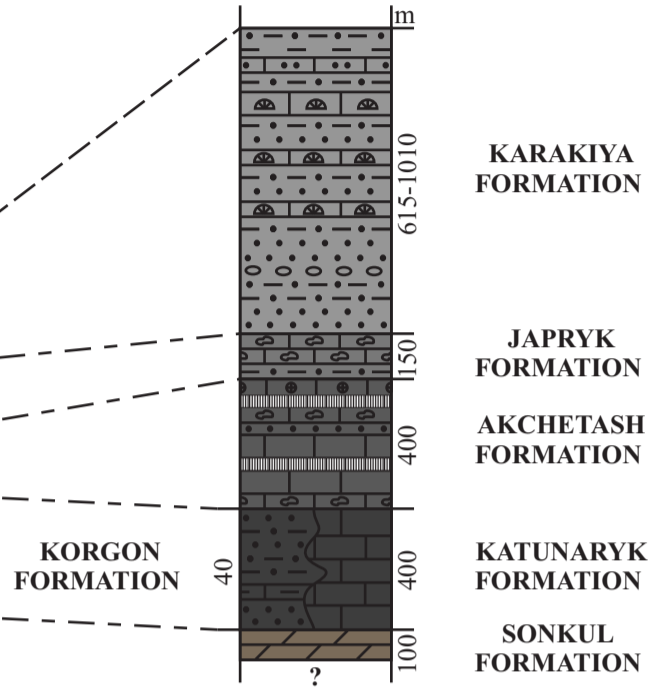
Karabulak nappe after A.V.Mikolaichuk (Orlov et al., 1979)
